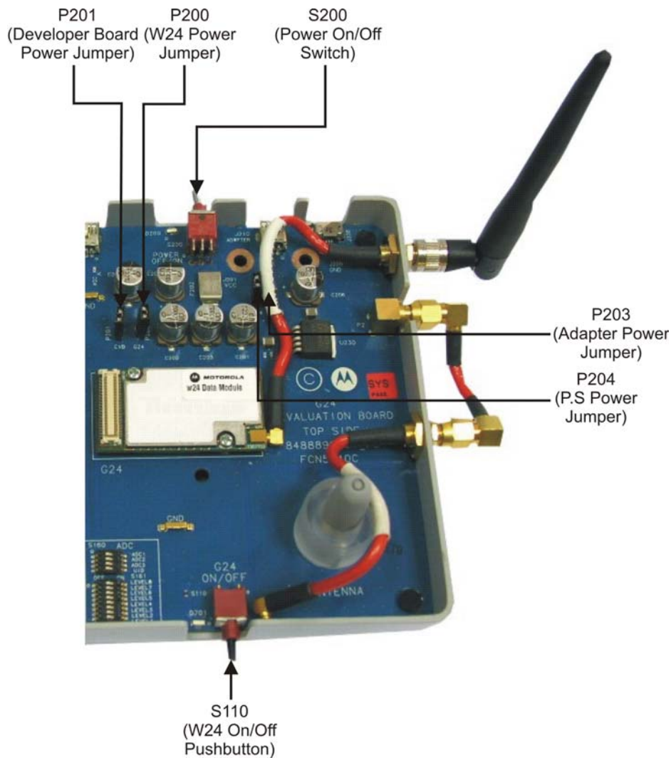
Figure 2-18: Jumpers and Switches on Developer Board
