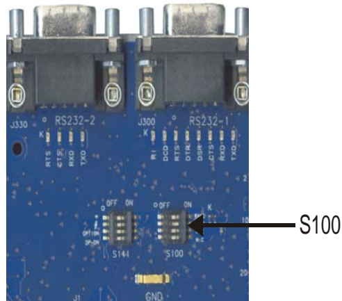
Figure 2-16: S100 Switches
