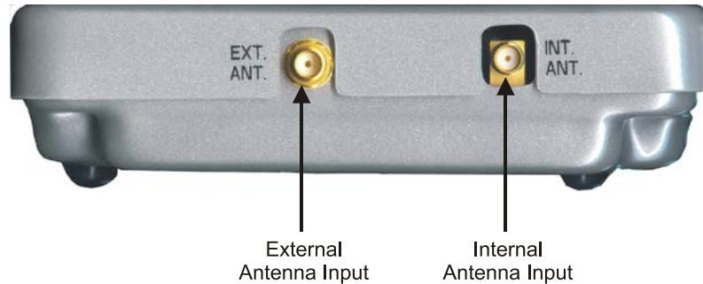
Figure 2-10: Antenna Connectors (external)
