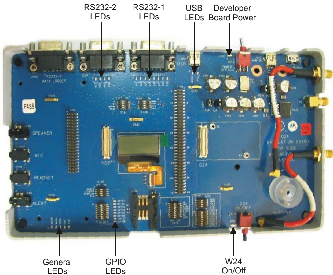
Figure 2-19: LEDs on Developer Board
