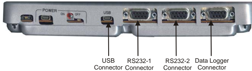
Figure 2-9: USB, RS232-1, RS232-2 and Data Logger Connectors
