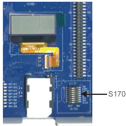
Figure 2-14: S170 Switches
