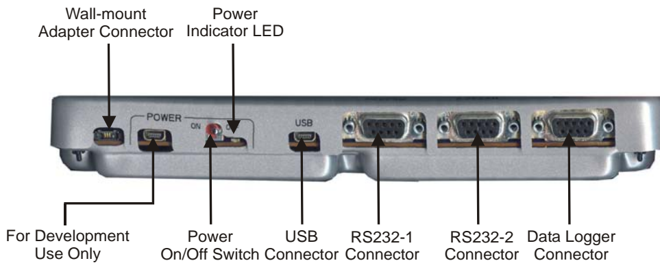
Figure 1-4: W24 Developer's Kit—Rear View with Cover
