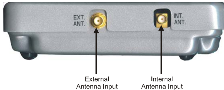
Figure 1-5: W24 Developer's Kit—Right Side View with Cover
