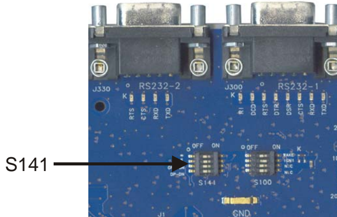
Figure 2-15: S141 Switches
