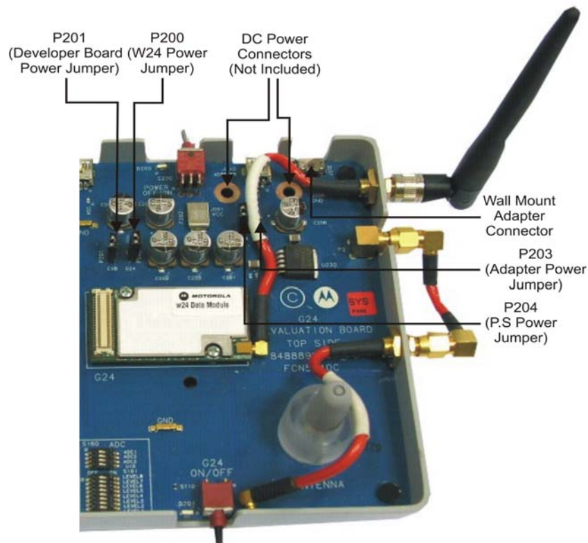
Figure 2-6: Power Supply Connectors, Jumpers and Switches
