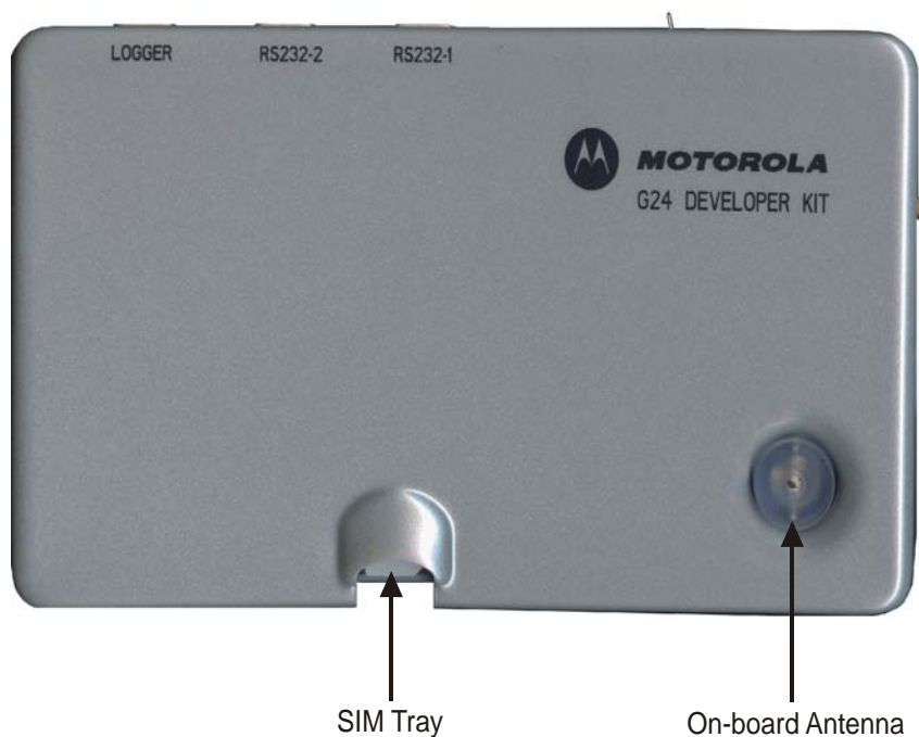
Figure 1-1: W24 Developer's Kit—Top View with Cover
