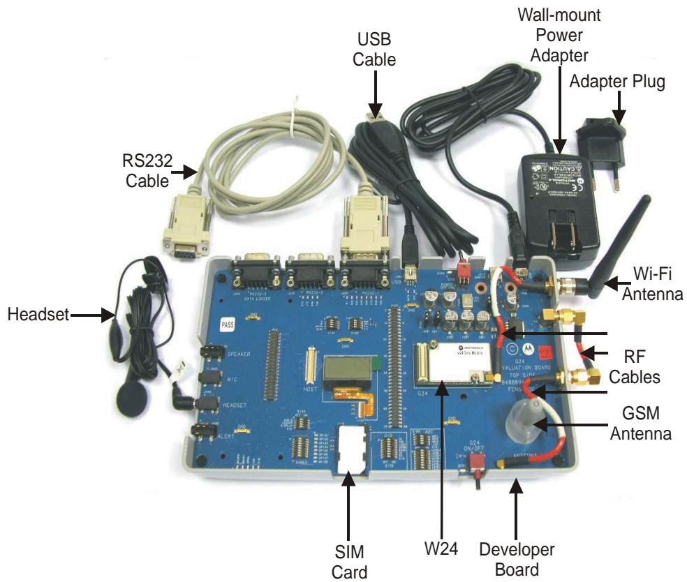
Figure 1-6: W24 Developer's Kit with Board, W24 and Accessories
