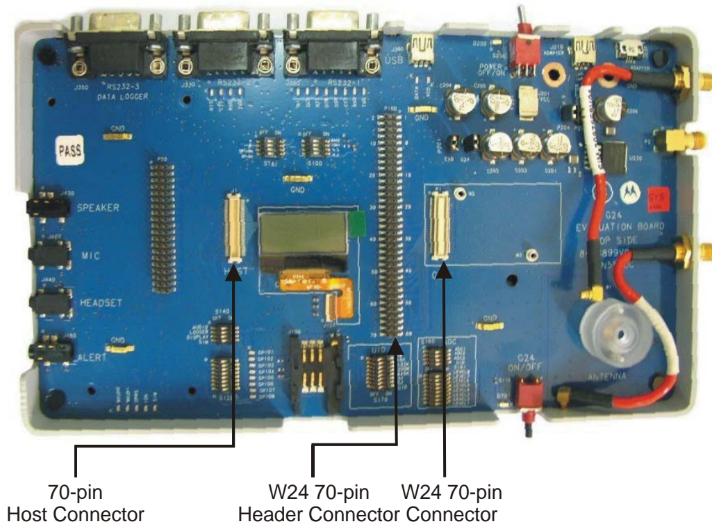
Figure 2-17: 70-pin Connectors
