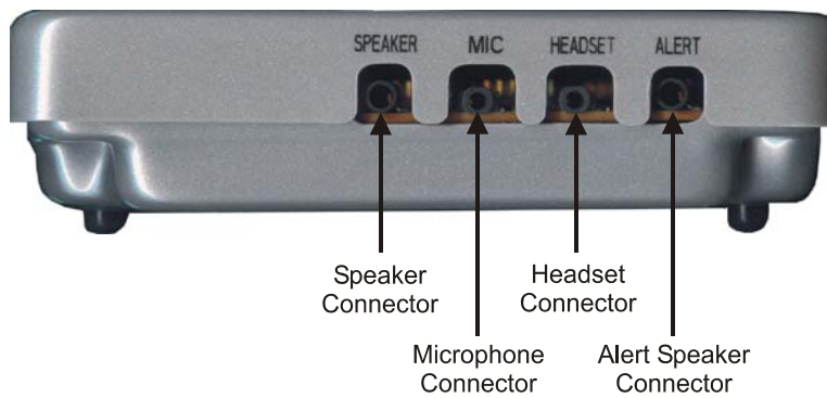
Figure 1-3: W24 Developer's Kit—Left Side View with Cover
