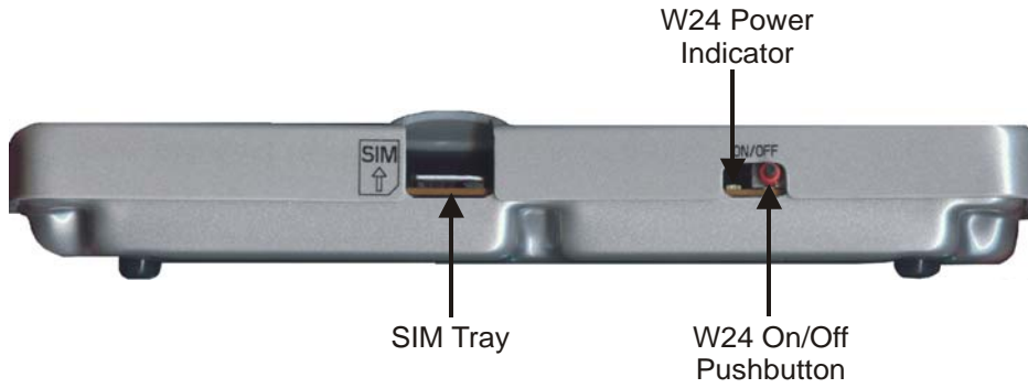
Figure 1-2: W24 Developer's Kit—Front View with Cover
