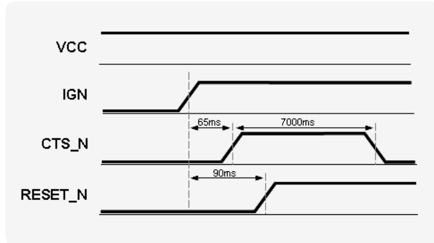
Figure 2-5: IGN Power On Timing
